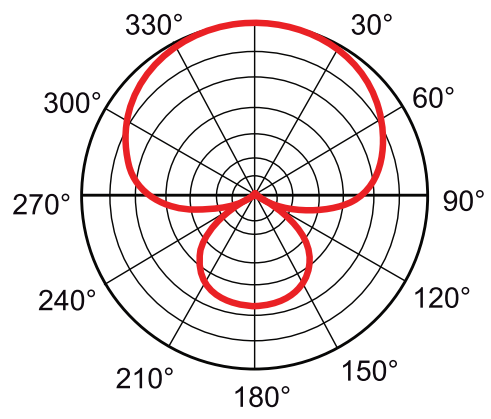
Supercardioid Polar Pattern
